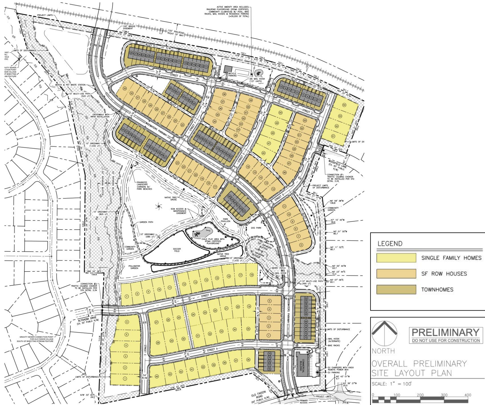
Figure 14: Concept Site Plan
