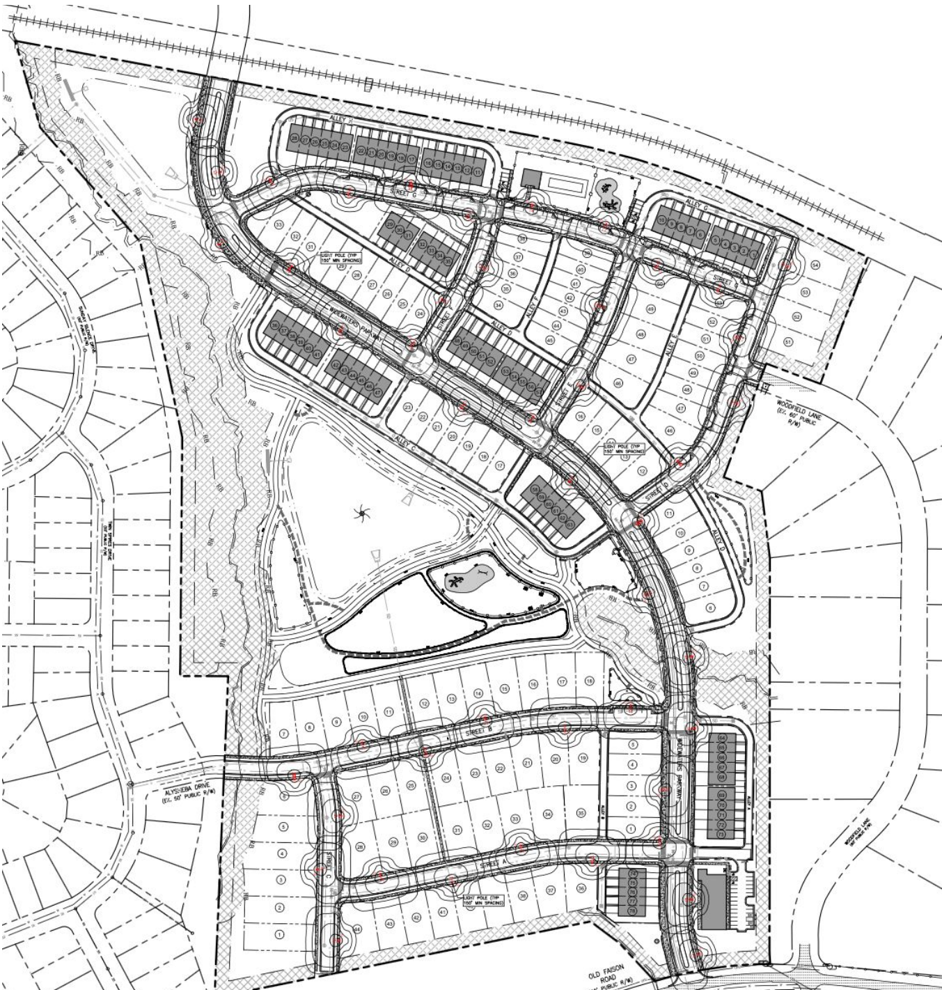
Figure 18: Lighting Plan
