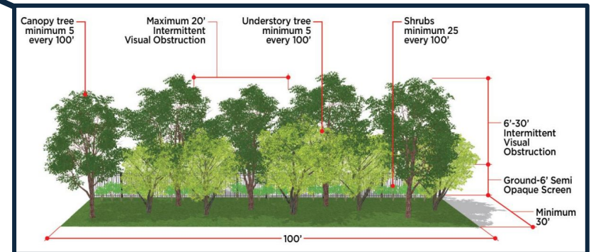
Figure 24: Type C Buffer Yard Standards from Knightdale UDO.
