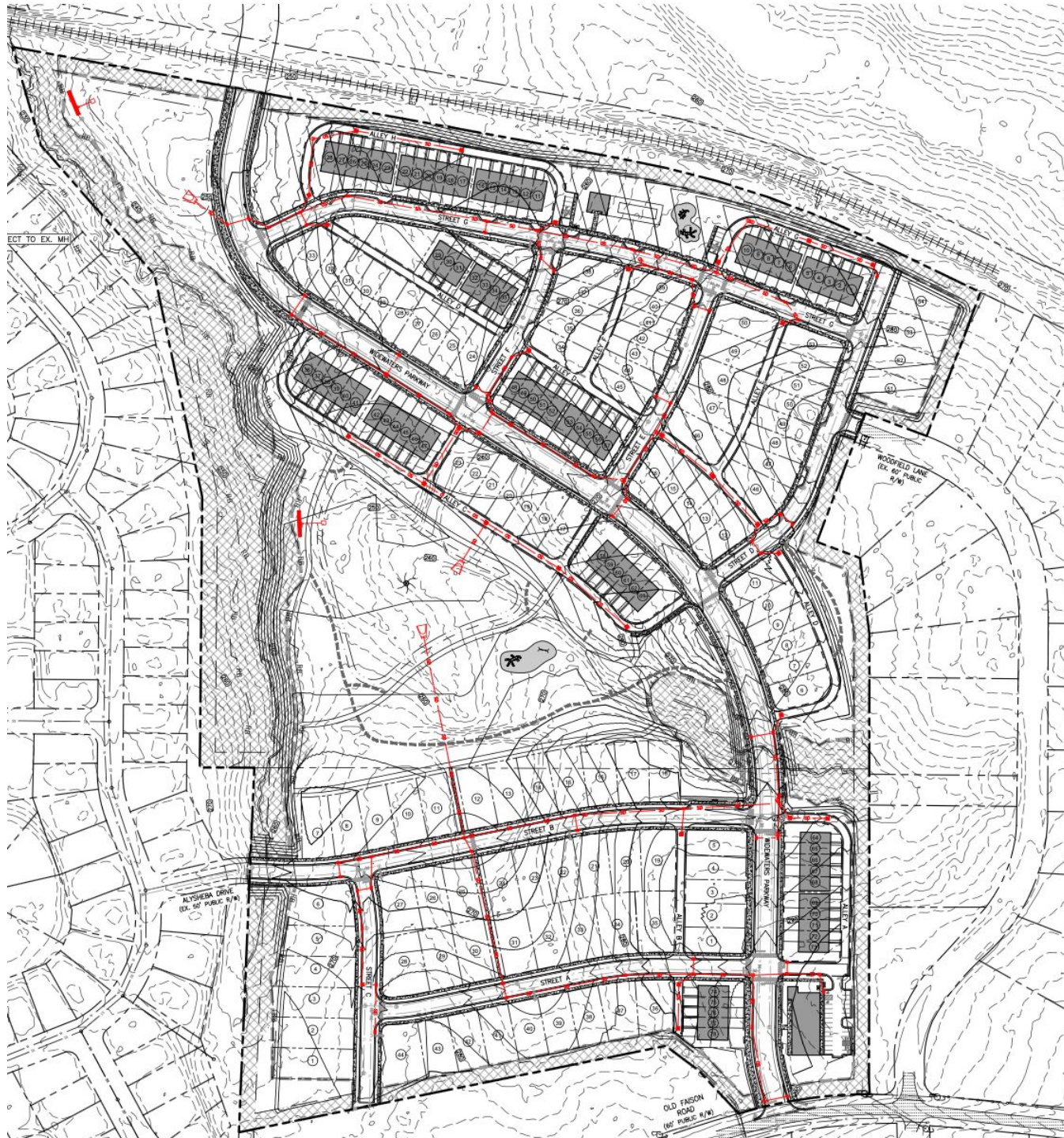
Figure 15: Stormwater Plan
