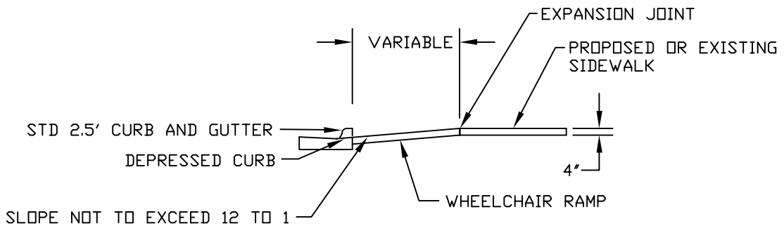
SECTION B-B
