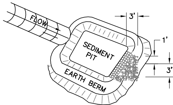
PERSPECTIVE VIEW
