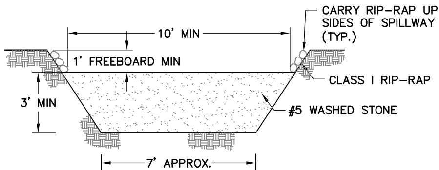
SECTION THROUGH BERM & FILTER
