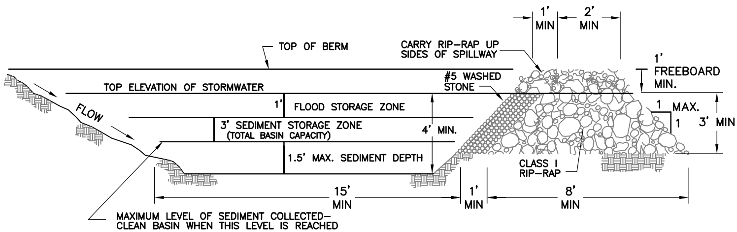
SECTION THROUGH BASIN & FILTER
