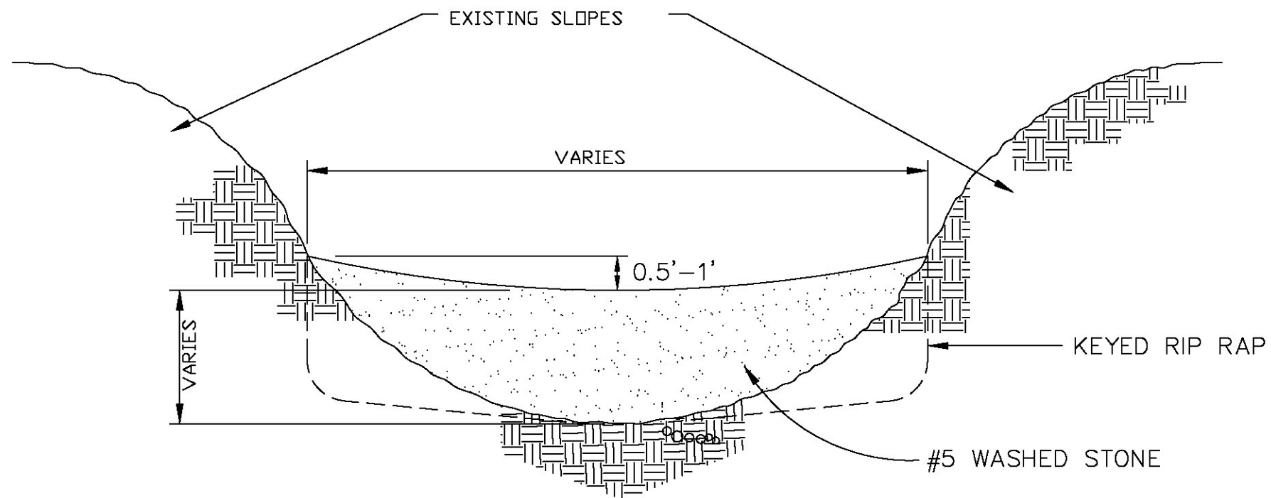
FRONT VIEW
