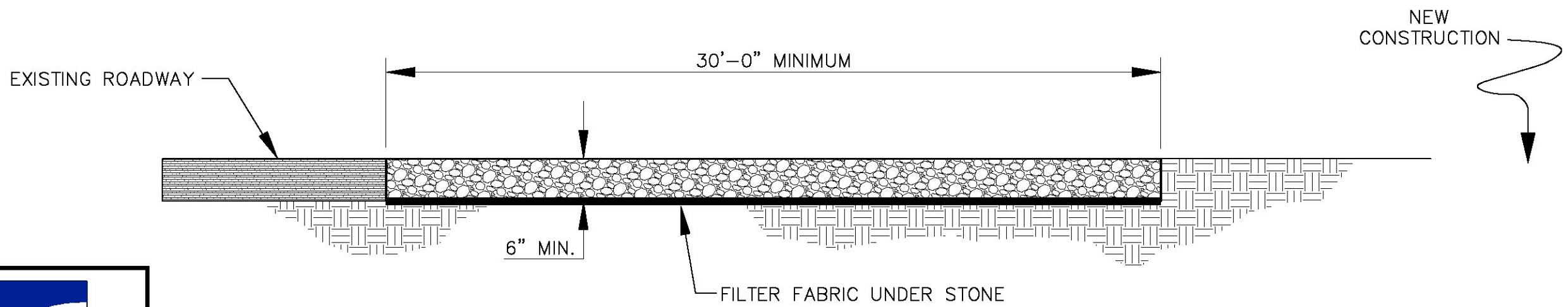
CROSS SECTION
