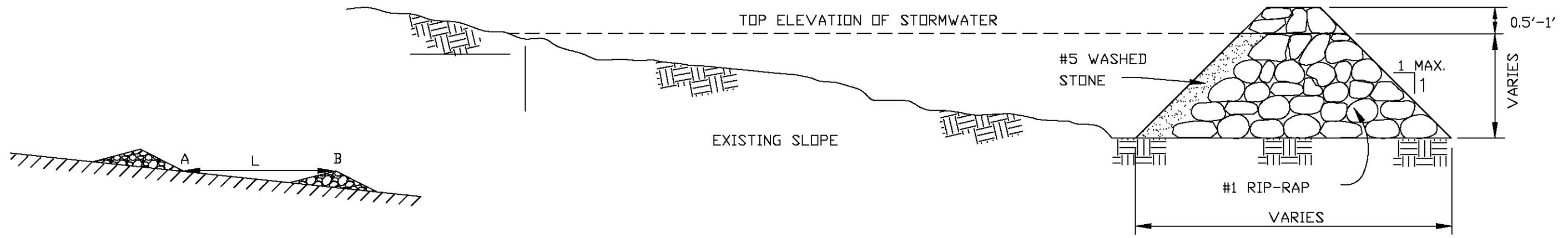
SIDE VIEW
