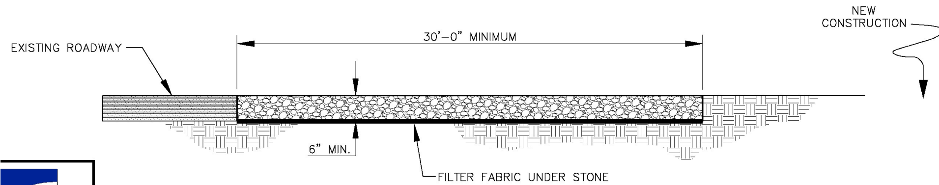
CROSS SECTION
