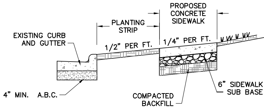
TYPICAL SECTION
